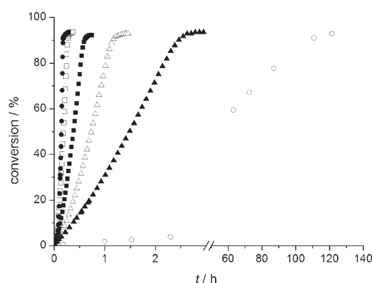
Figure 1. Effect of temperature on the decomposition of formic acid in a closed (batch) system: 25 °C (○) (125 mM Ru), 70 °C (▲), 80 °C (△), 90 °C (■), 100 °C (□), 120 °C (●) (22 mM Ru); [\text{Ru}(\text{H}_2\text{O})_6](\text{tos})_2 , 2 equiv TPPTS, 4 M \text{HCOOH}/\text{HCOONa} (9:1), 2.5 mL \text{H}_2\text{O}/\text{D}_2\text{O} (1:1); addition of 0.38 mL \text{HCOOH} for recycling.
